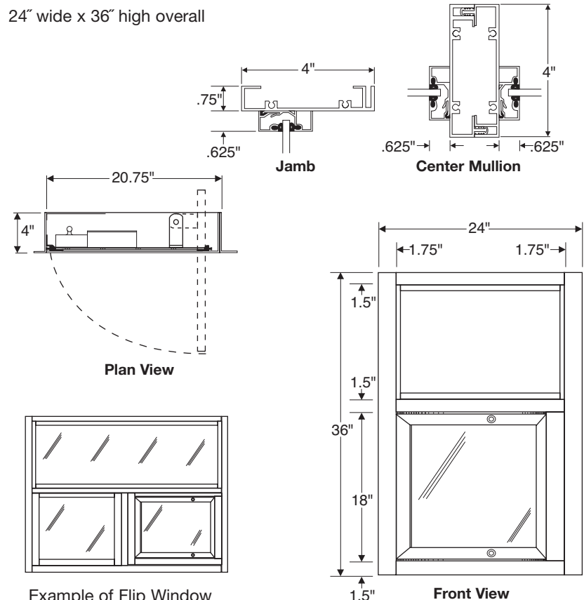
Example of Flip Window below full width transom.
