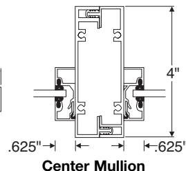
Center Mullion
